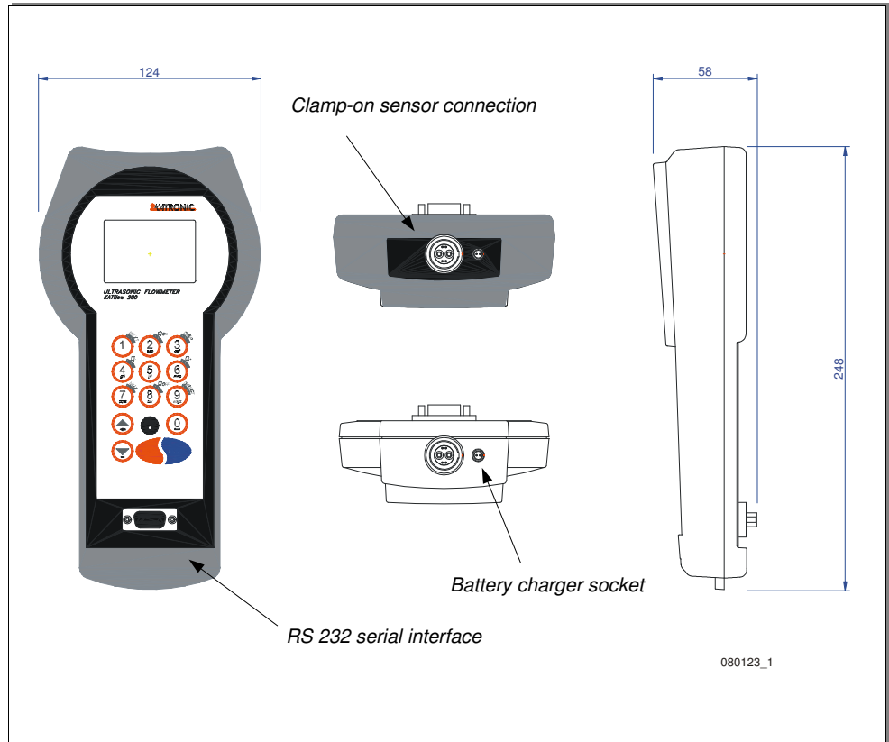
Drawing 1: Outline dimensions KATflow 200
